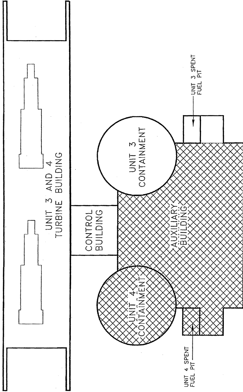
TURKEY POINT UNIT 4 SITE PLAN
